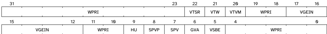
Figure 79. Hypervisor status register ( hstatus ) when HSXLEN =32
