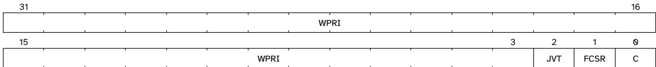
Figure 37. Supervisor State Enable 0 Register (sstateen0)
