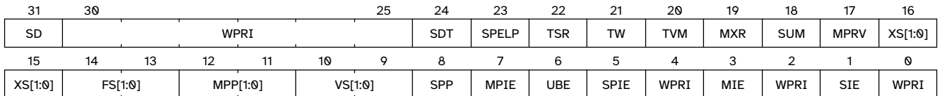
Figure 7. Machine-mode status ( mstatus ) register for RV32
