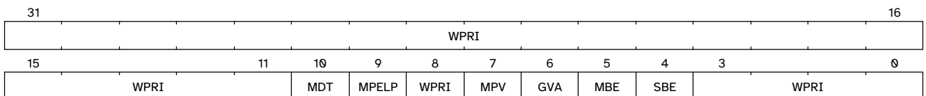
Figure 9. Additional machine-mode status ( mstatush ) register for RV32.
