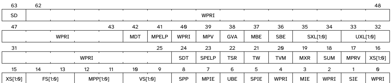
Figure 8. Machine-mode status ( mstatus ) register for RV64
