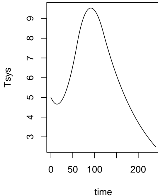
fortran/rodeo
